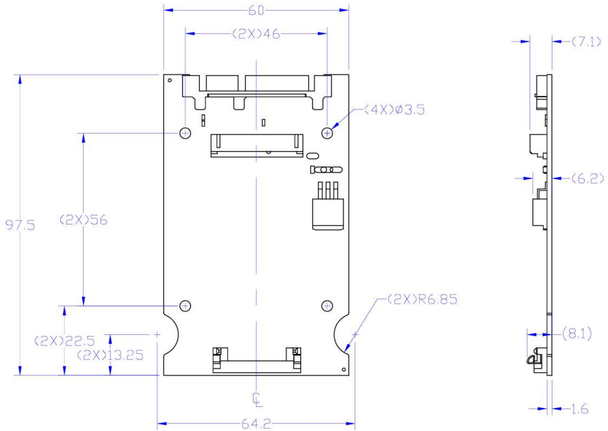
Figure 1: TB1527 adapter with dimensions (measured in mm)
